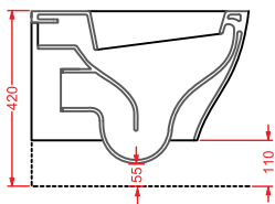
TEB003 TEN bidet terra floor bidet
