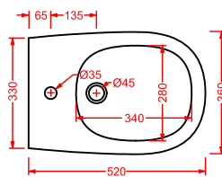
TEB001 TEN bidet terra filomuro back to wall bidet
