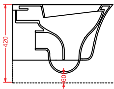
CWB002 COW bidet terra back to wall bidet
