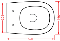
TEV003 TEN vaso sospeso wall-hung WC
