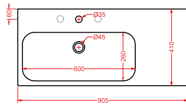
BKL002 BLOCK lavabo sospeso/appoggio 90 wall-hung/countertop washbasin 90
