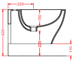
TEV002 TEN vaso terra filomuro back to wall WC
