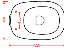
TEV001 TEN vaso terra scarico "S" "S" trap floor WC
