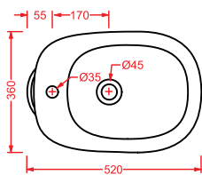
TEB003 TEN bidet terra floor bidet
