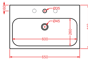
BKL001 BLOCK lavabo sospeso/appoggio 65 wall-hung/countertop washbasin 65
