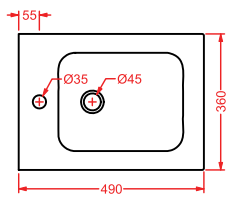
BKB002 BLOCK bidet terra back to wall bidet
