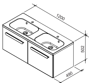
SD 1200 Chrome
