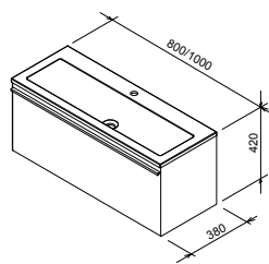
SD Clear 800/1000
