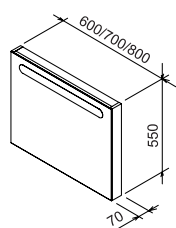
Mirrors Chrome 600 / 700 / 800
