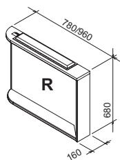
M 780/960 L/R
