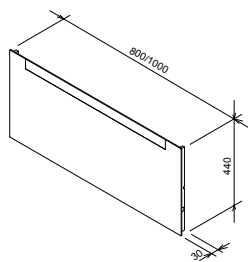
Mirror Clear 800/1000
