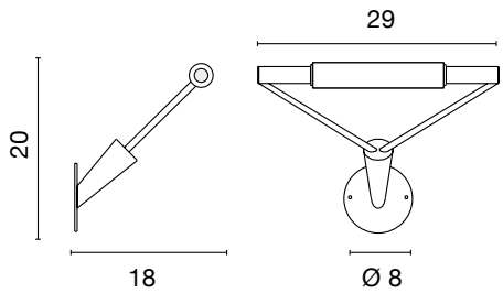
4138 1 kg 160W R7s ECO F IP 40 .22 .32
