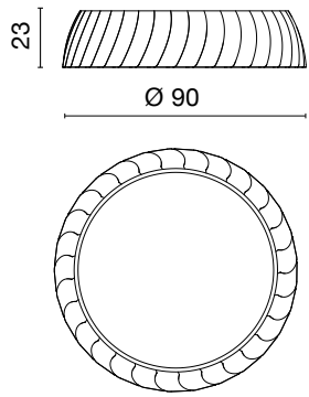
5537 4 kg Led 33W 4246lm 3000K F .01/WW
